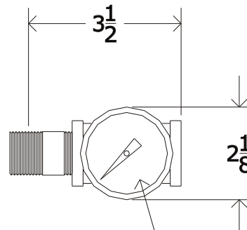
0-300PSI GAUGE AND INSTALLATION TEE
