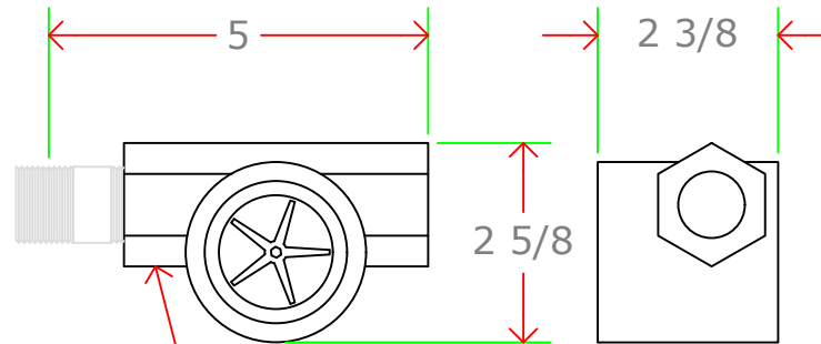
BRASS SIGHT FLOW INDICATOR
